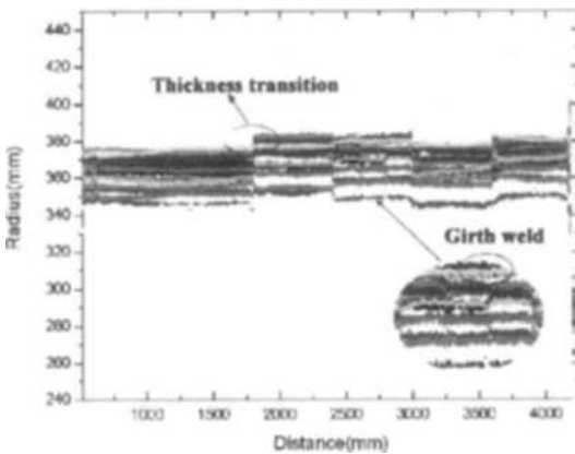
Fig. 11 Experimental result in pull-rig facility
