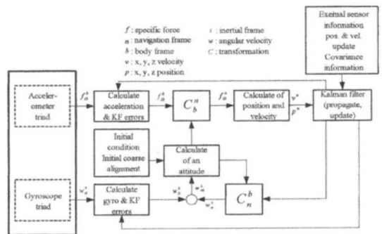
Fig. 6 SIMU processing
