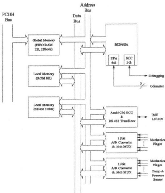
Fig. 4 Scheme of DPU of the geometry PIG
