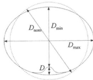
Fig. 5 Computation of the feature size
